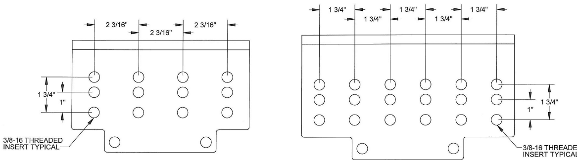
Optional Load Cable Detail For Disconnects Rated 800 through 2400 AMP
