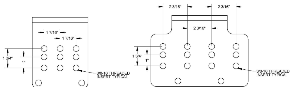
Optional Load Cable Detail For Disconnects Rated 100 through 750 AMP
